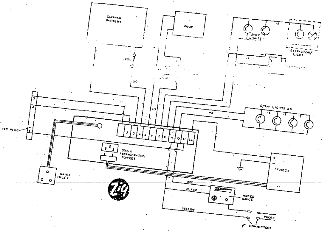
Figure 3. Suggested wiring diagram for C. F. 2000
